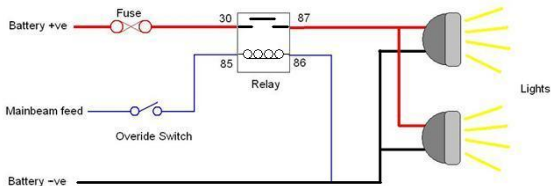
Wiring Diagram for Negative Earth
